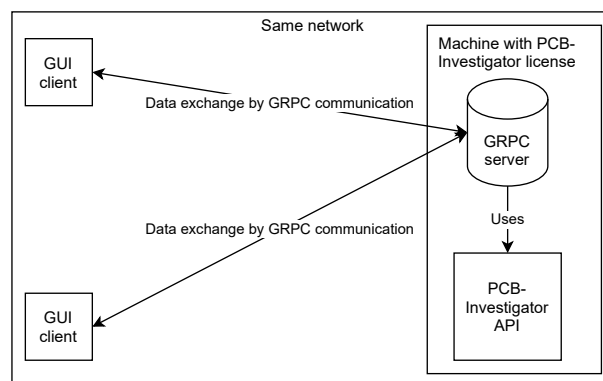
Figure 3.1.: Client-server structure of the planned software
